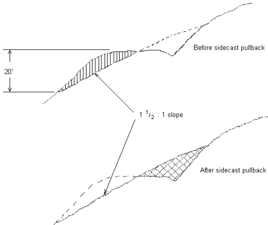
TYPICAL CROSS SECTION VIEW OF SIDECAST PULLBACK AND ROAD REALIGNMENT
